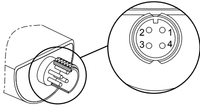
Fig. 4 Electrical connections
