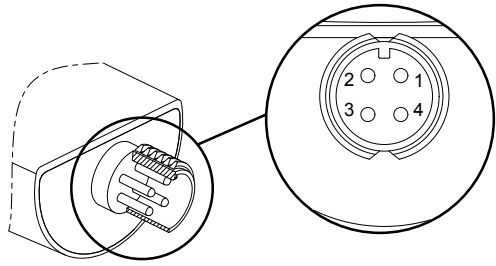
Fig. 72 Electrical connections
