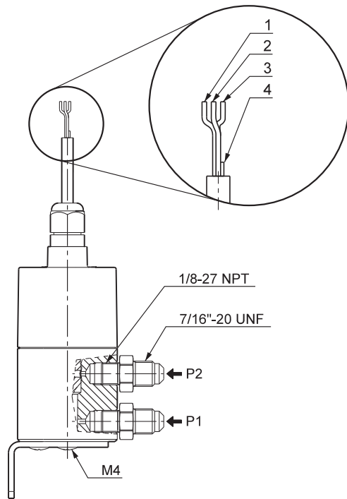
Fig. 46 Electrical connections
